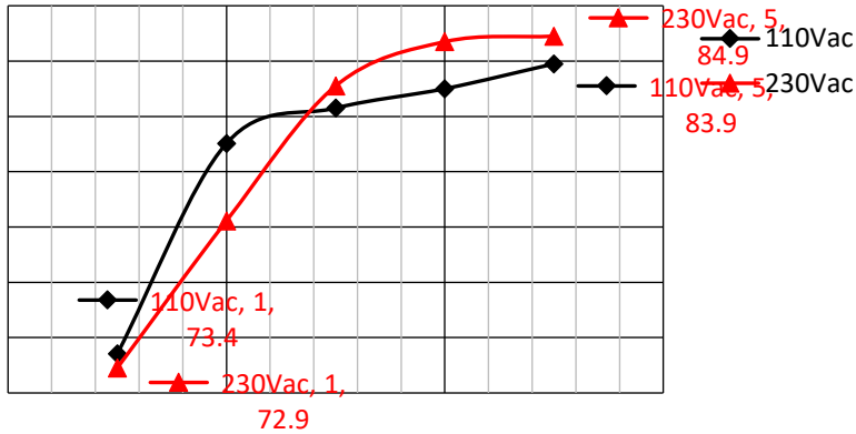
(%) Efficiency Vs. Input Voltage & Output Current
