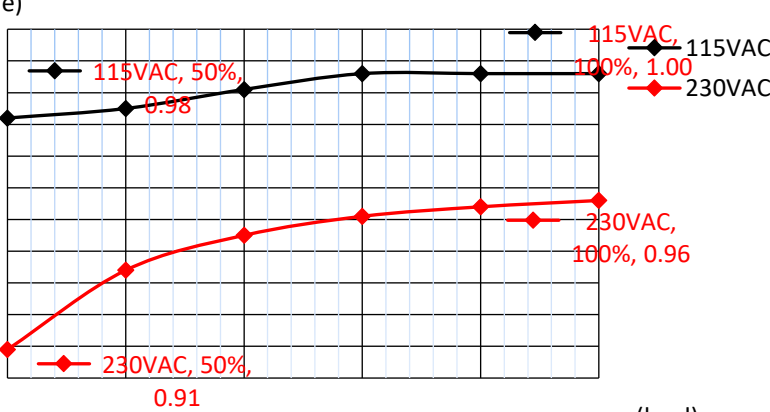
(value) PFC value Vs. Output Load Current
